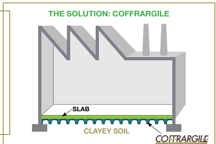
Behavior in the case of soil shrinkage
